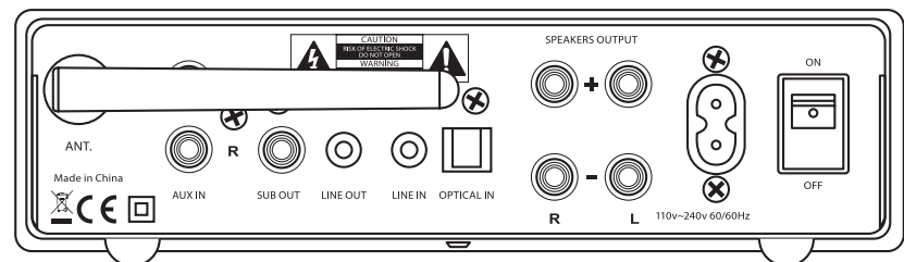
BACK VIEW
